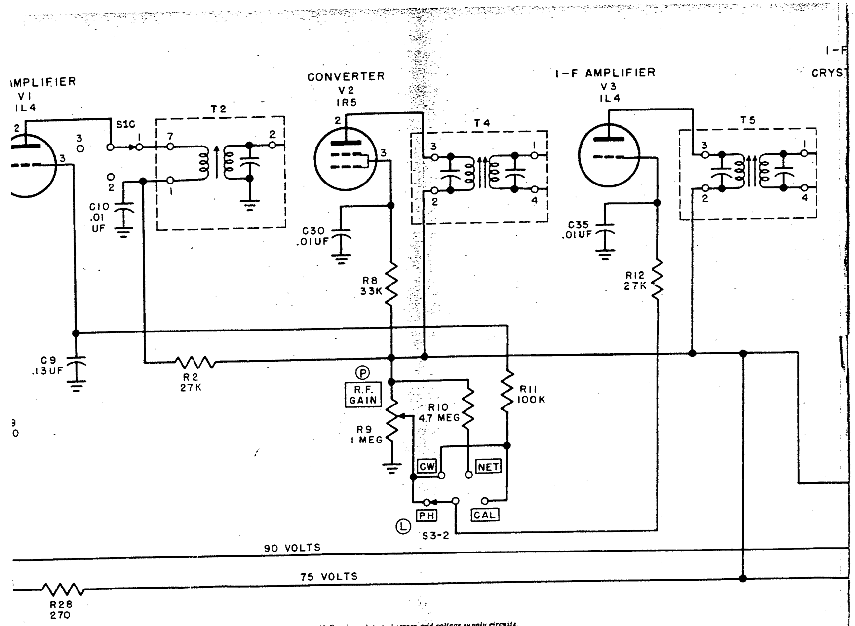
Figure 65 Receiver plate and screen grid voltage supply circuits.
